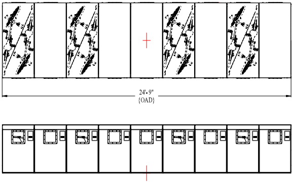
EcoPark DV {M18} Locker Bank (9) Units = (18) Bike Capacity
