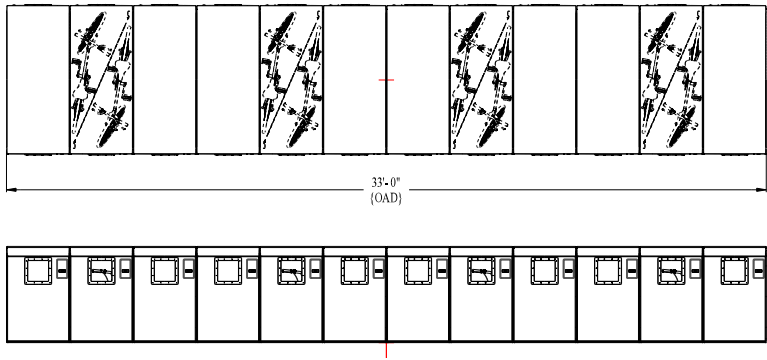
EcoPark DV {M24} Locker Bank (12) Units = (24) Bike Capacity
