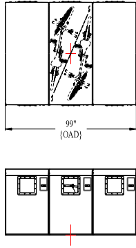
EcoPark DV {M06} Locker Bank (3) Units = (6) Bike Capacity
