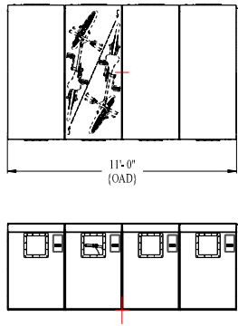
ProPark DV {M08} Locker Bank (4) Units = (8) Bike Capacity
