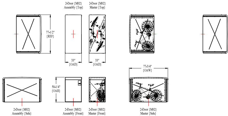
EcoPark SM {M02} Locker Bank (1) Units = (2) Bike Capacity
