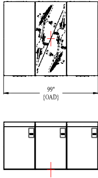
EcoPark SM {M06} Locker Bank (3) Units = (6) Bike Capacity
