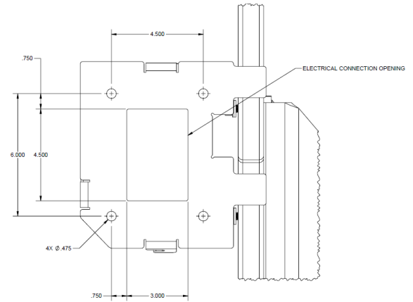
Bottom anchoring plate dimensions
