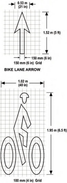
Figure 12. Recommended bike lane pavement parking
