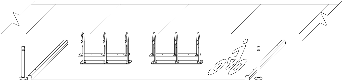
ISOMETRIC VIEW
