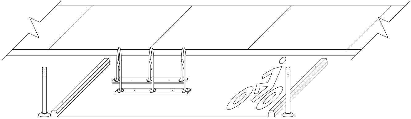
ISOMETRIC VIEW
